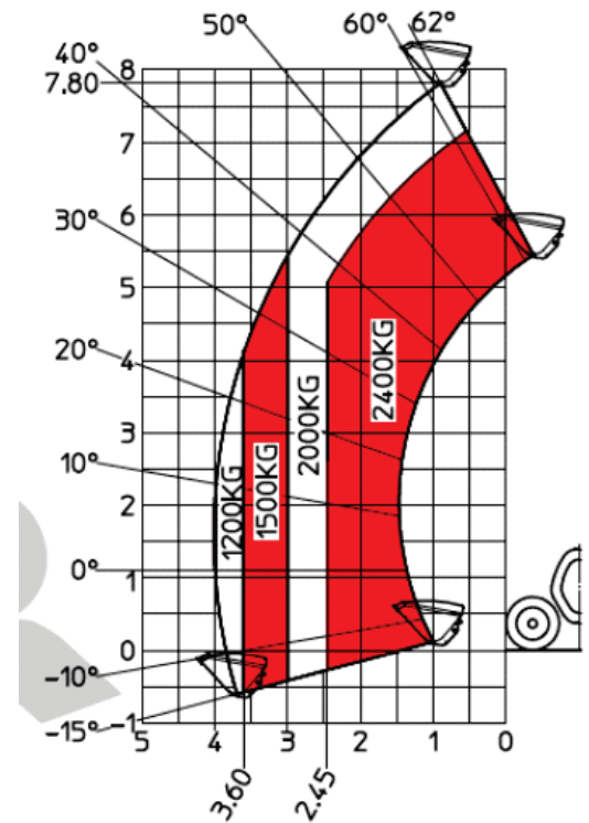
Load chart with 3 cu.m bucket.
